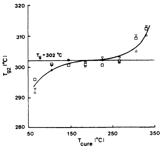
Fig. 9. T_{g2} vs. T_{\text{cure}} for the polyamic acid/polyimide system for 12 ( \Delta ), 24 ( \square ), and 96 ( \nabla ) h isothermal cure. The curve represents the general trend for the three time scales.
