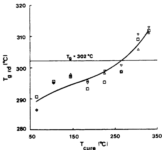
Fig. 8. T_{g \text{ rd}} vs. T_{\text{cure}} for the polyamic acid/polyimide system for 12 ( \Delta ), 24 ( \square ), and 96 ( \nabla ) h isothermal cure. The curve represents the general trend for the three time scales.
