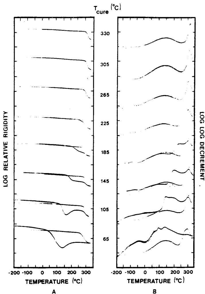
Fig. 4. TBA temperature scans of the polyamic acid/polyimide system after 24 h isothermal cure: relative rigidity (A) and logarithmic decrement (B) vs. temperature. Plots are shown for the temperature sequence: T_{\text{cure}} to -180 to 330 to -180^{\circ}\text{C} at 2^{\circ}\text{C}/\text{min} .
