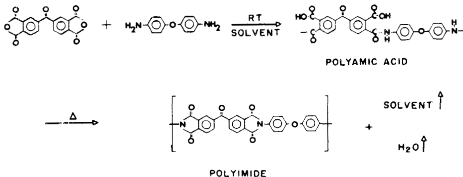
Fig. 2. Reaction scheme.
