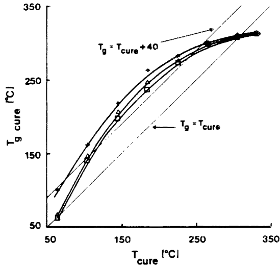
Fig. 13. T_{g \text{ cure}} vs. T_{\text{cure}} for the polyamic acid/polyimide system for 12 ( \square ), 24 ( \Delta ), and 96 (+) h isothermal cure. The lines T_g = T_{\text{cure}} and T_g = T_{\text{cure}} + 40^\circ\text{C} are also shown.
