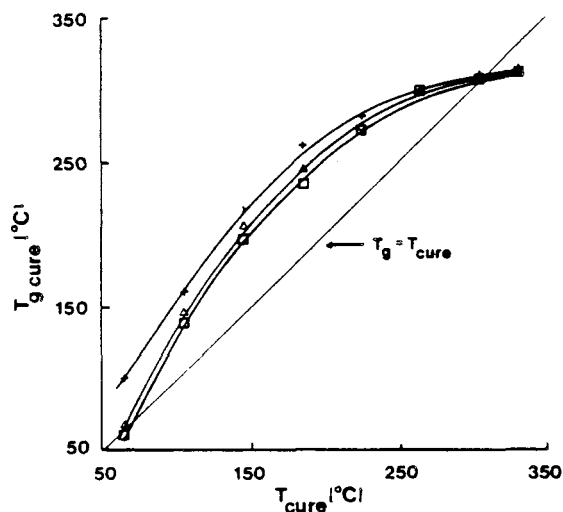
Fig. 7. T_g vs. T_{cure} for the polyamic acid/polyimide system for 12 (□), 24 (Δ), and 96 (+) h isothermal cure. The line T_g = T_{cure} is also shown.
