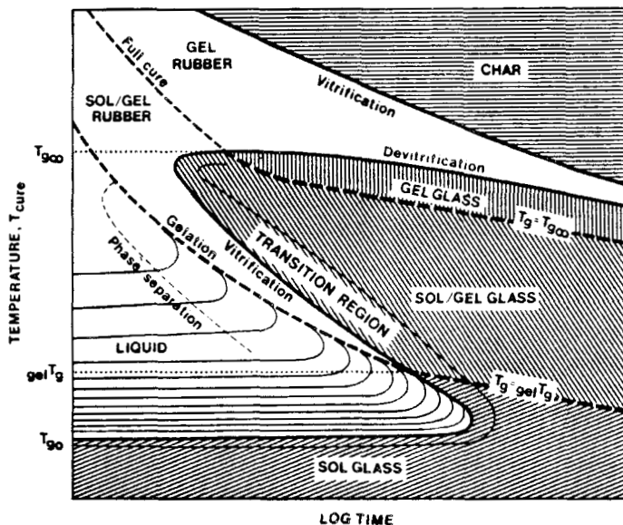
Fig. 1. Generalized time-temperature-transformation (TTT) isothermal cure diagram for epoxy thermosetting systems, showing three critical temperatures, i.e., T_{g\infty} , gel T_g , and T_{g0} , and the distinct states of matter, i.e., liquid, sol/gel rubber, gel rubber (elastomer), gelled glass, ungelled (or sol) glass, and char. The full-cure line, i.e., T_g = T_{g\infty} , divides the gelled glass region into two parts: sol/gel glass and gel (fully cured) glass. Phase separation, as in rubber-modified systems, occurs prior to gelation. Successive isoviscous contours shown in the liquid region differ by a factor of 10. The transition region corresponds to the half-width of the glass transition. T_{g0} , gel T_g and T_{g\infty} are the glass transition temperatures of the reactants, the material at the composition corresponding to gelation, and the fully cured system, respectively.
