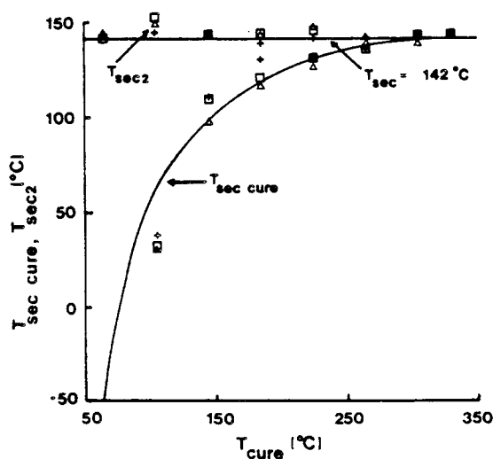
Fig. 10. T_{\text{sec cure}} and T_{\text{sec}2} vs. T_{\text{cure}} for the polyamic acid/polyimide system for 12 ( \Delta ), 24 ( \square ), and 96 (+) h isothermal cure. The solid lines show general trends.
