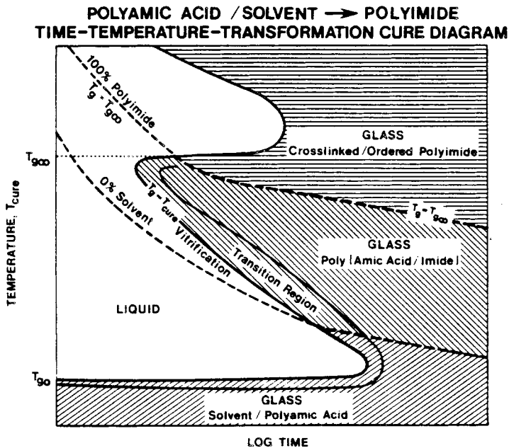
Fig. 16. Schematic TTT isothermal cure diagram for the polyamic acid/solvent/polyimide system.
