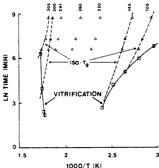
Fig. 15. The TTT cure diagram presented as \ln time vs. 1/T_{\text{cure}} (K): (□) vitrification; (Δ) iso- T_g .
