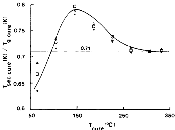
Fig. 11. T_{\text{sec cure}} (\text{K})/T_{\text{g cure}} (\text{K}) vs. T_{\text{cure}} for the polyamic acid/polyimide system for 12 (+), 24 (□), and 96 (Δ) h isothermal cure. The solid curve shows the general trend. The ratio approaches a stable value of 0.71 for T_{\text{cure}} > 265^{\circ}\text{C} .
