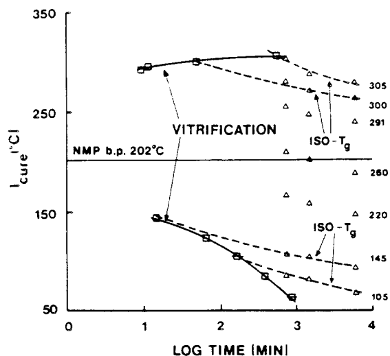
Fig. 12. The TTT cure diagram for the polyamic acid/polyimide system including iso- T_g lines ( \Delta ) obtained using data from Figure 7.
