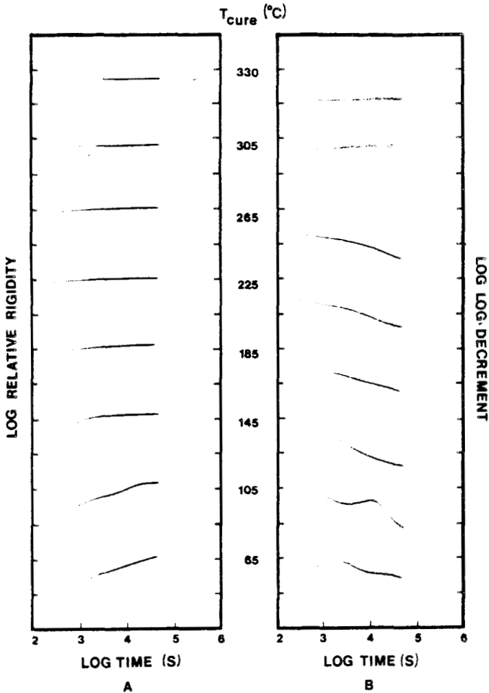
Fig. 3. TBA isothermal spectra for the polyamic acid/polyimide system: relative rigidity (A) and logarithmic decrement (B) vs. time for the 24 h time scale.
